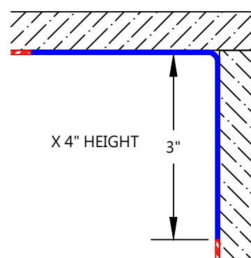
CRDA-64-IC INSIDE CORNER
