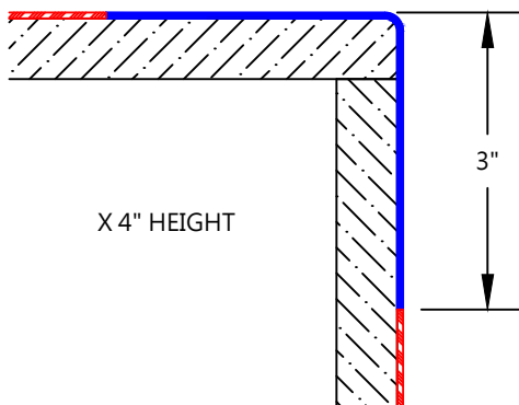
CRDA-64-OC OUTSIDE CORNER
