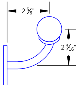
HR-15B3 BRACKET • LONG ARM SCREW MOUNT
