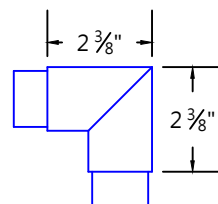
HR-15MC MITRED STYLE 90° CORNER
