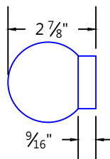
HR-15B 90° BALL TYPE END CAP
