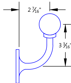
HR-15T BRACKET • SHORT ARM SCREW MOUNT
