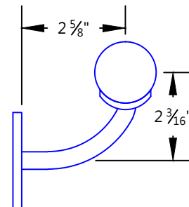
HR-15B3 BRACKET • LONG ARM SCREW MOUNT
